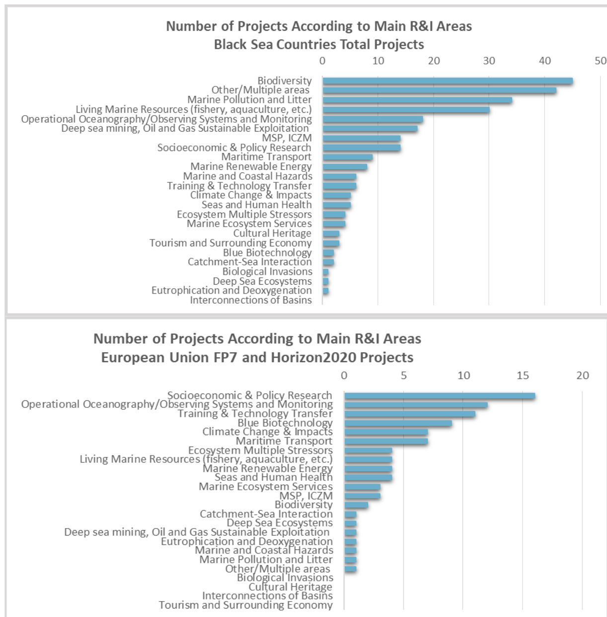
Figure 3 Marine research projects targeting the Black Sea
